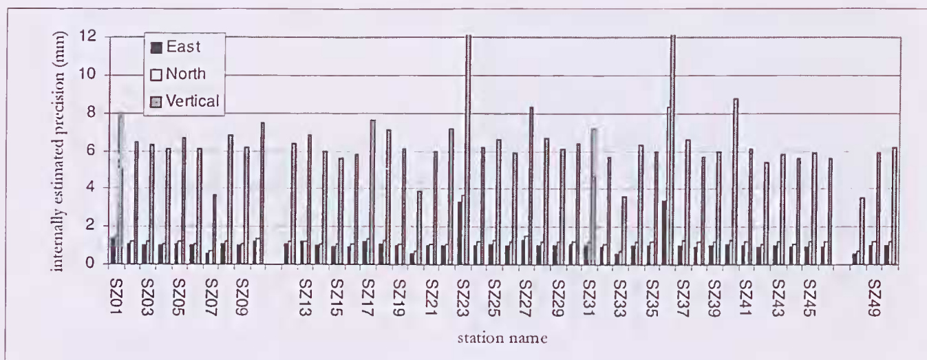
Figure 4. Internally estimated precision ( 1\sigma ) of the epoch-one GPS-derived coordinates (ITRF2000 epoch 2002.37) of the 48-point network across the SWSZ (units in mm) [SZ11 and SZ47 were not placed]
